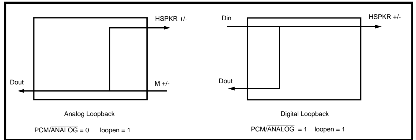
Figure 8 - Loopback Signal Flows
