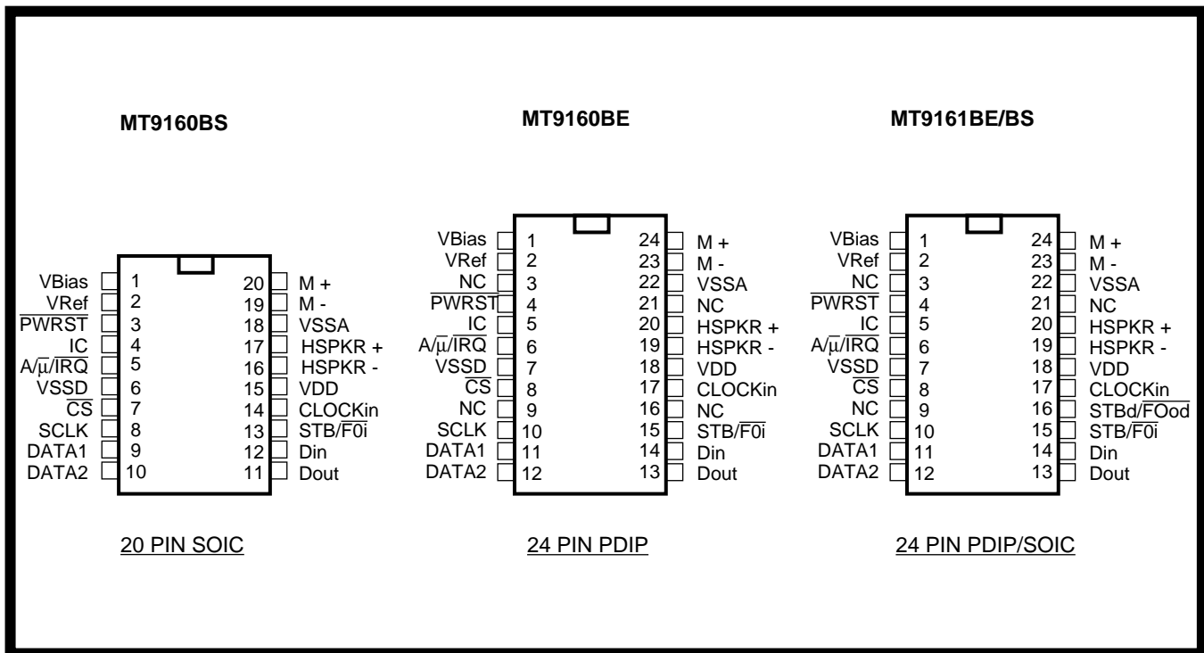
Figure 2 - Pin Connections
